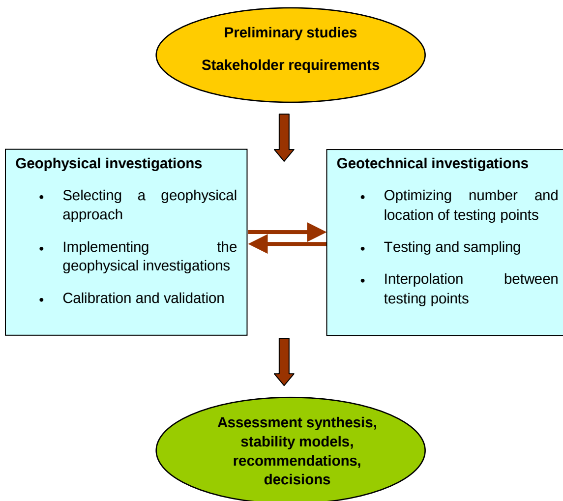
Figure 2.7 Condition assessment methodology: this diagram presents a close-up and an alternative to Fig. 1.1 in the sense that geophysical and geotechnical investigations are conducted in a fully interactive process (with mutual expectations and benefits).
