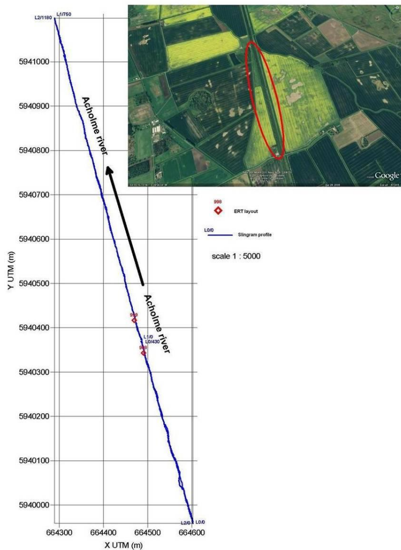
Figure 2.23 Slingram profile and detailed ERT measurement at Site B
