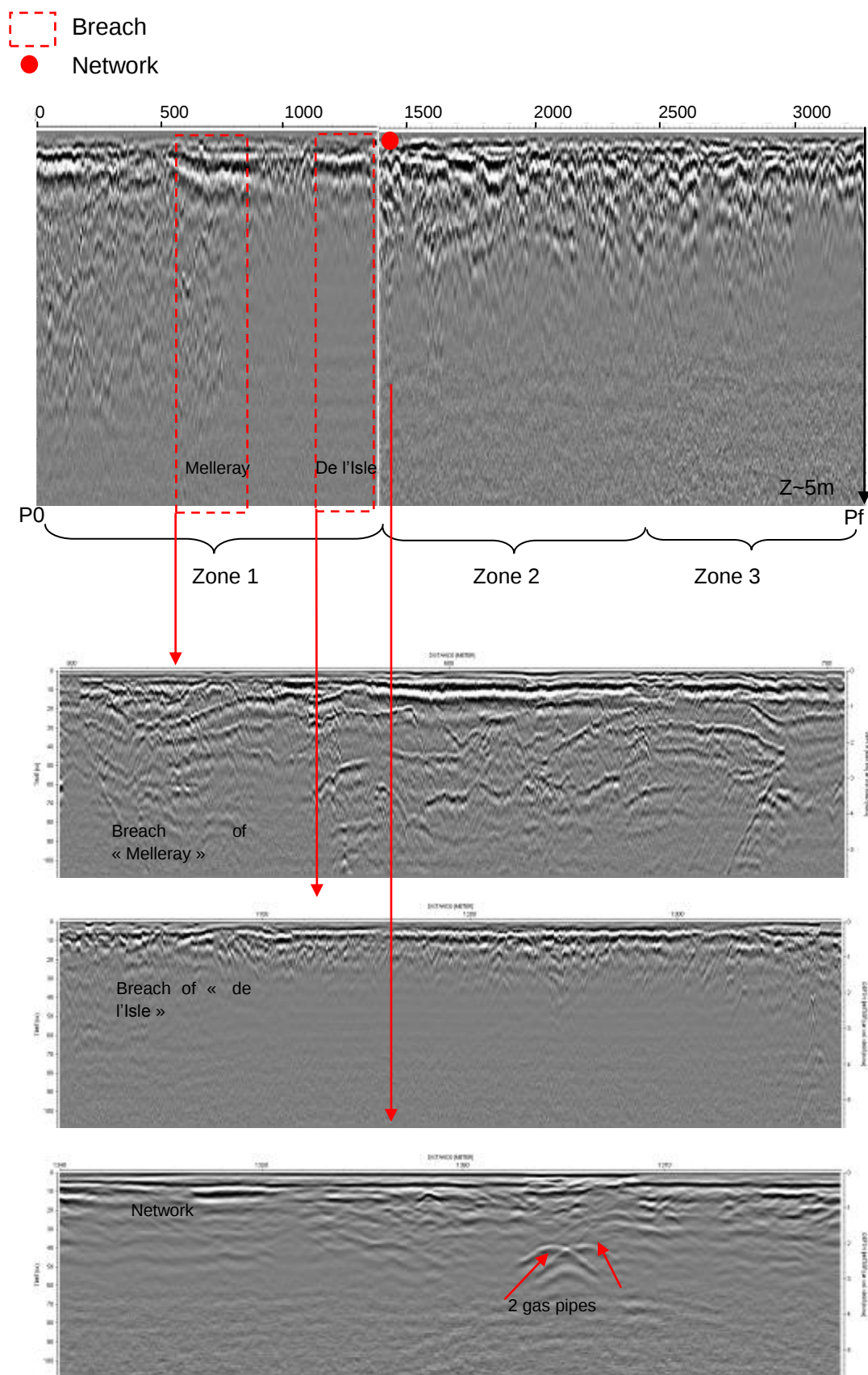
Figure 2.14 GPR measurements at 200 MHz. On top, whole profile and zoom on the breaches and the gas network.
