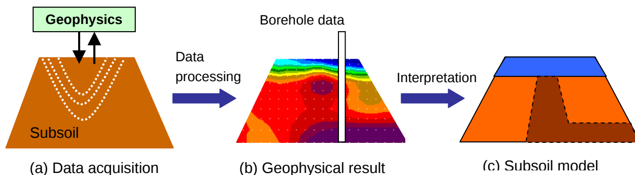
Figure 2.1 General scheme of a geophysical investigation process: (a) geophysical data acquisition, (b) geophysical parameter graph, map or cross-section and (c) subsoil structure model or geotechnical property distribution.
