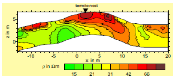
Figure 2.26 Example of ERT measurement on dike (Henig and al., 2011)
