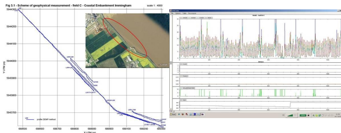
Figure 2.24 Slingram profile and results at the Site C
