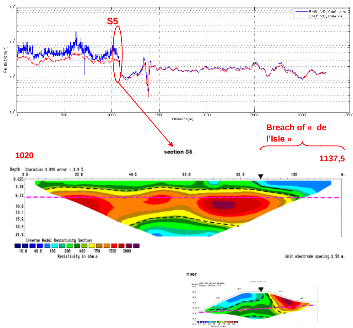
Figure 2.15 Slingram and ERT measurements at the transition with a known old breach.
